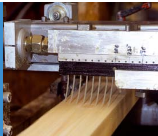
Application head of OEST Ecopur G glue dosing unit for 1-component polyurethane glue.
